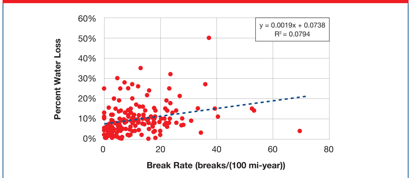
FIGURE 37: PERCENT WATER LOSS VERSUS UTILITY BREAK RATES
